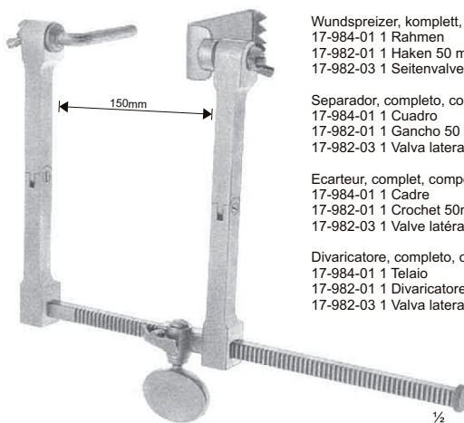
SCOVILLE-HAVERFIELD 17-984-00
