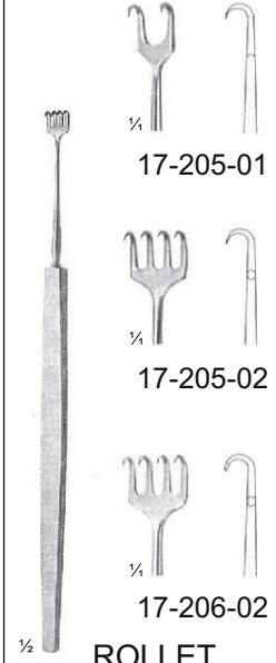
ROLLET 17-205-01 17-206-02 14 cm, 5½"
